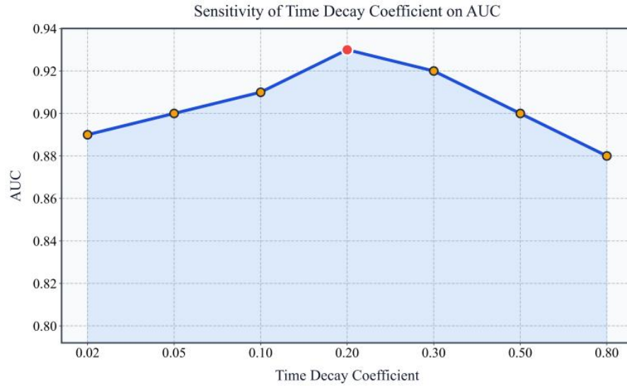
Figure 2. Time decay factor on AUC
