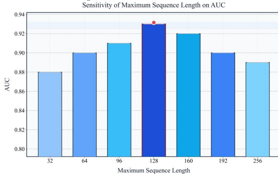
Figure 3. The effect of maximum sequence length sensitivity on AUC
