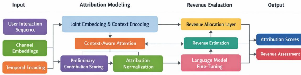
Figure 1. Overall model architecture
